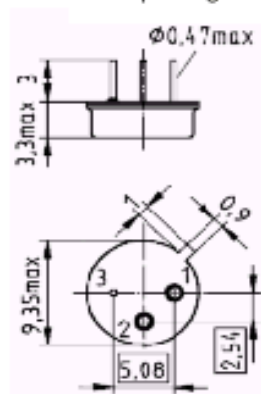
Metal package TO39
